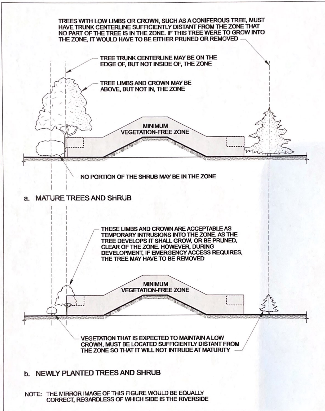
Figure A-2. Proper Application of the Vegetation-Free Zone.
