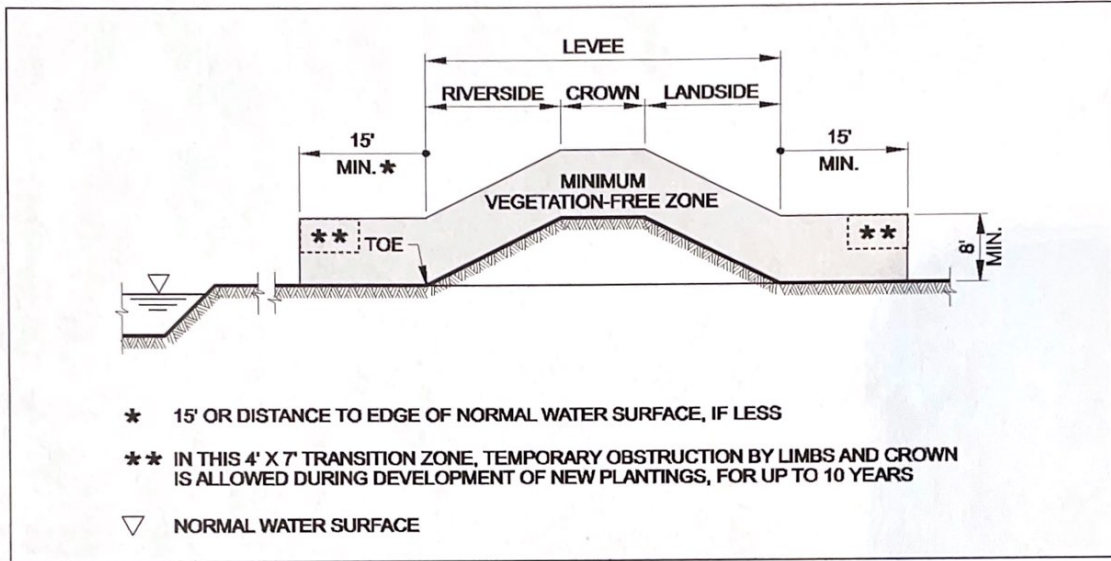
Figure A-1. Levee Section – Basic.
